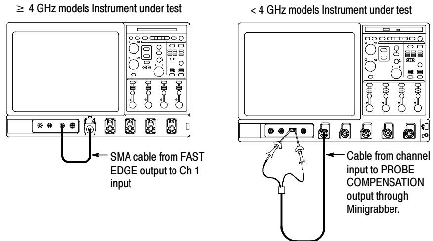
Figure 2-6: Setup for the file system test
