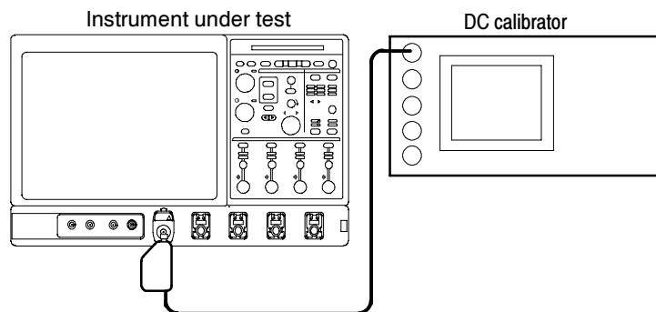
Figure 2-11: Initial test hookup
